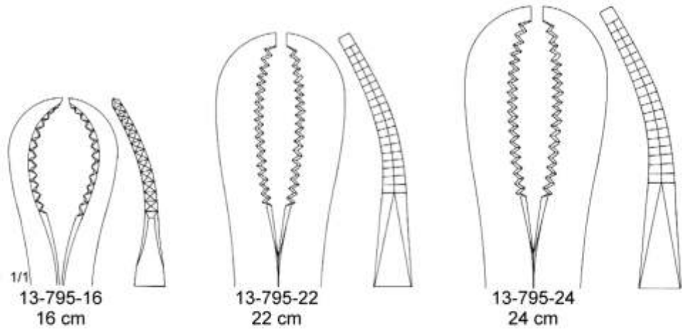
Reposition forceps with thread fixation
