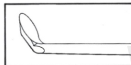
BC-21-534 2mm diameter blade, angled up 45 degrees Overall length 168 mm, 6.6 inches
