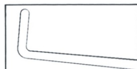
BC-21-486 1 mm long tip Angled left 90 degrees Malleable shaft, angled 8 degrees 53 mm from angle to tip Overall length 168 mm, 6.6 inches
