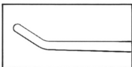
BC-21-548 Blunt 2 mm long tip Angled 35 degrees Overall length 171 mm, 6.7 inches
